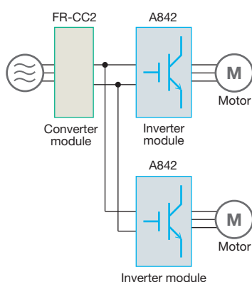
Common bus
