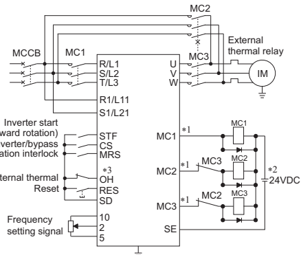
Electronic bypass sequence connection diagram (standard model)
