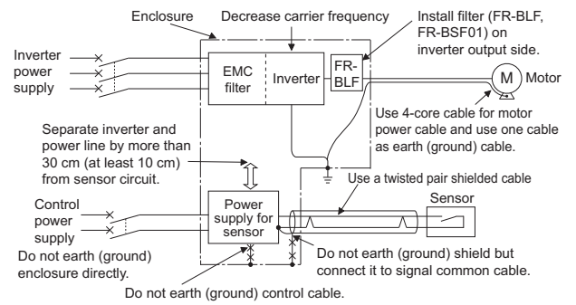
EMI measure example
