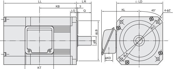
MM-CF□B (With an electromagnetic brake)
